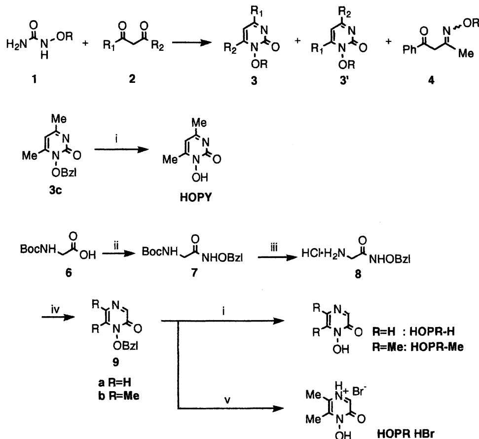
Scheme 1. Reagents and conditions: i) \text{H}_2/10\% Pd-C in MeOH, r.t., 20 min.; ii) Isobutyl chloroformate/ \text{Et}_3\text{N}/\text{H}_2\text{NOBz} , -15^\circ\text{C} to r.t., overnight; iii) 4 M HCl in dioxane, 0^\circ\text{C} , 1 h; iv) Glyoxal for 9a or 2,3-butanedione for 9b /5 M NaOH, -30^\circ\text{C} to r.t., overnight; v) 30% HBr in AcOH, r.t., 2 h.
