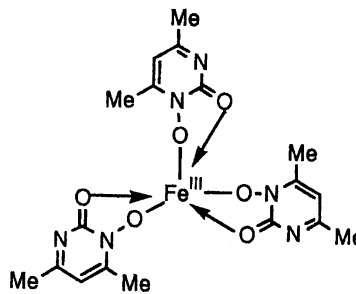
Fig. 3. Possible structure of the HOPY : \text{Fe(III)} = 3 : 1 complex.
